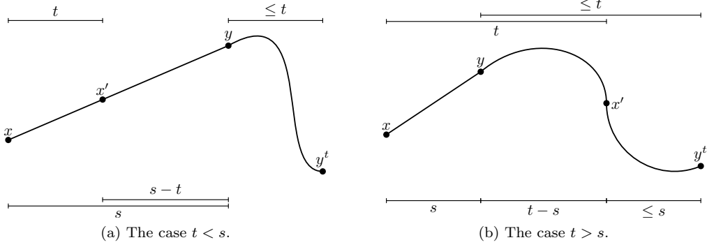
Figure 3: Sketches for the situations in the proof of Lemma 23. Indicated is always the path length according to l in Definition 3.
